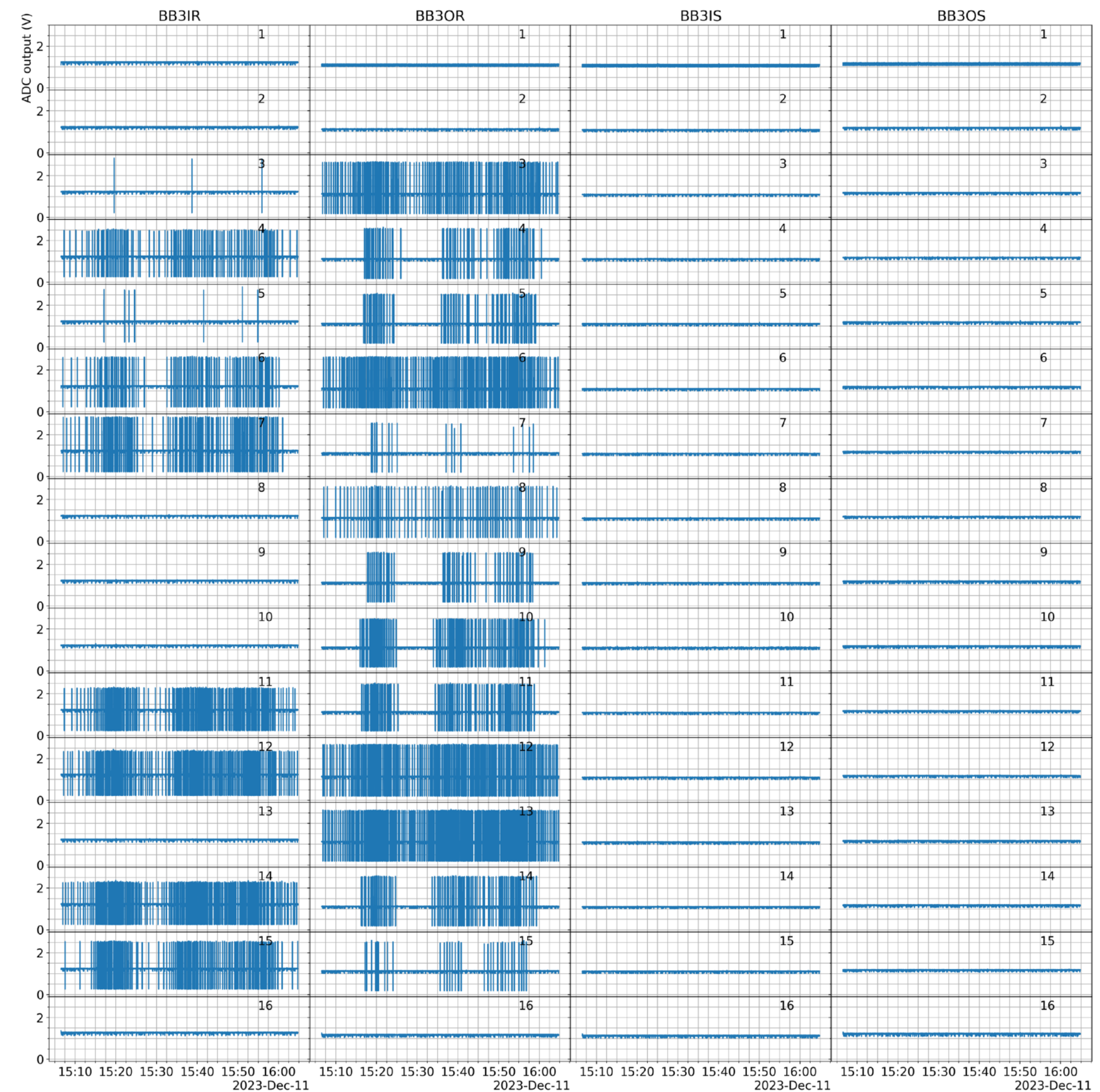
pi1(BB3) oscilloscope mode
