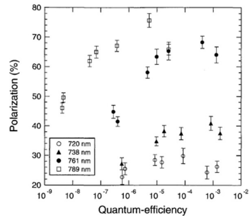
Fig. 2. QE dependence of the polarization at 720.1, 737.8, 761.1 and 788.7 nm.
