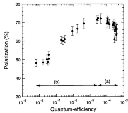
Fig. 1. QE dependence of the polarization at a wavelength of 778.5 nm.
