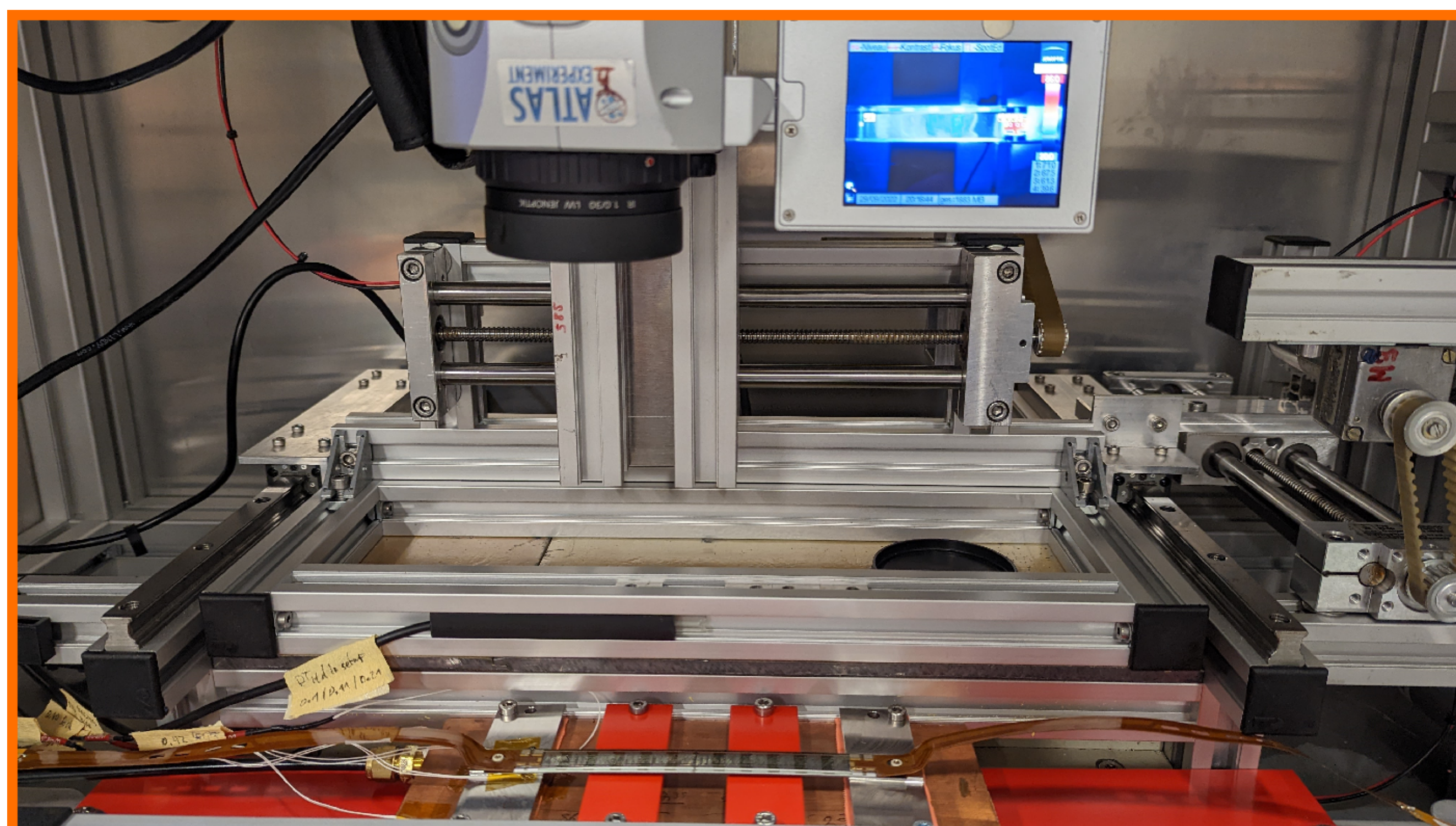
Single module thermal studies with infrared camera
