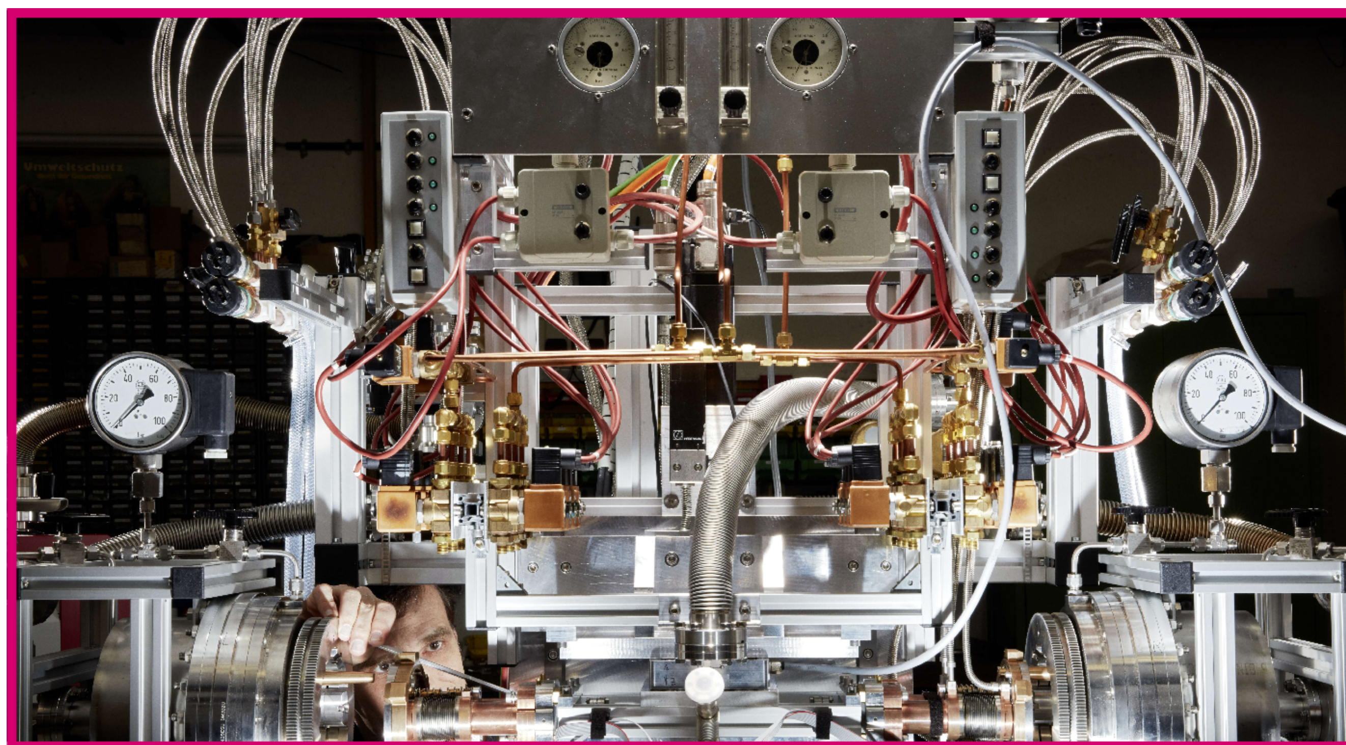
Remote vacuum connections, a machine-detector interface
