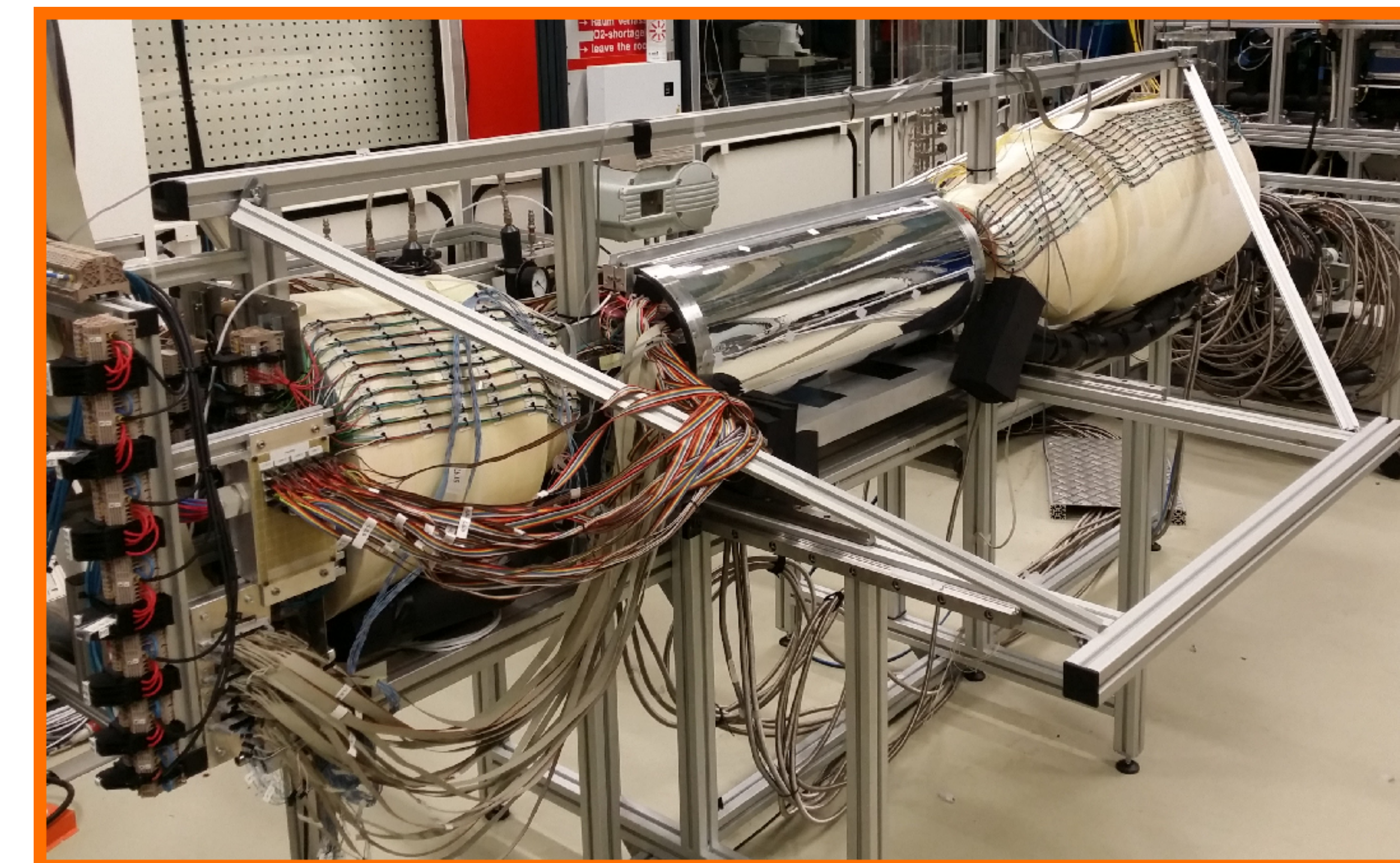
Real-size mockup for thermal studies
