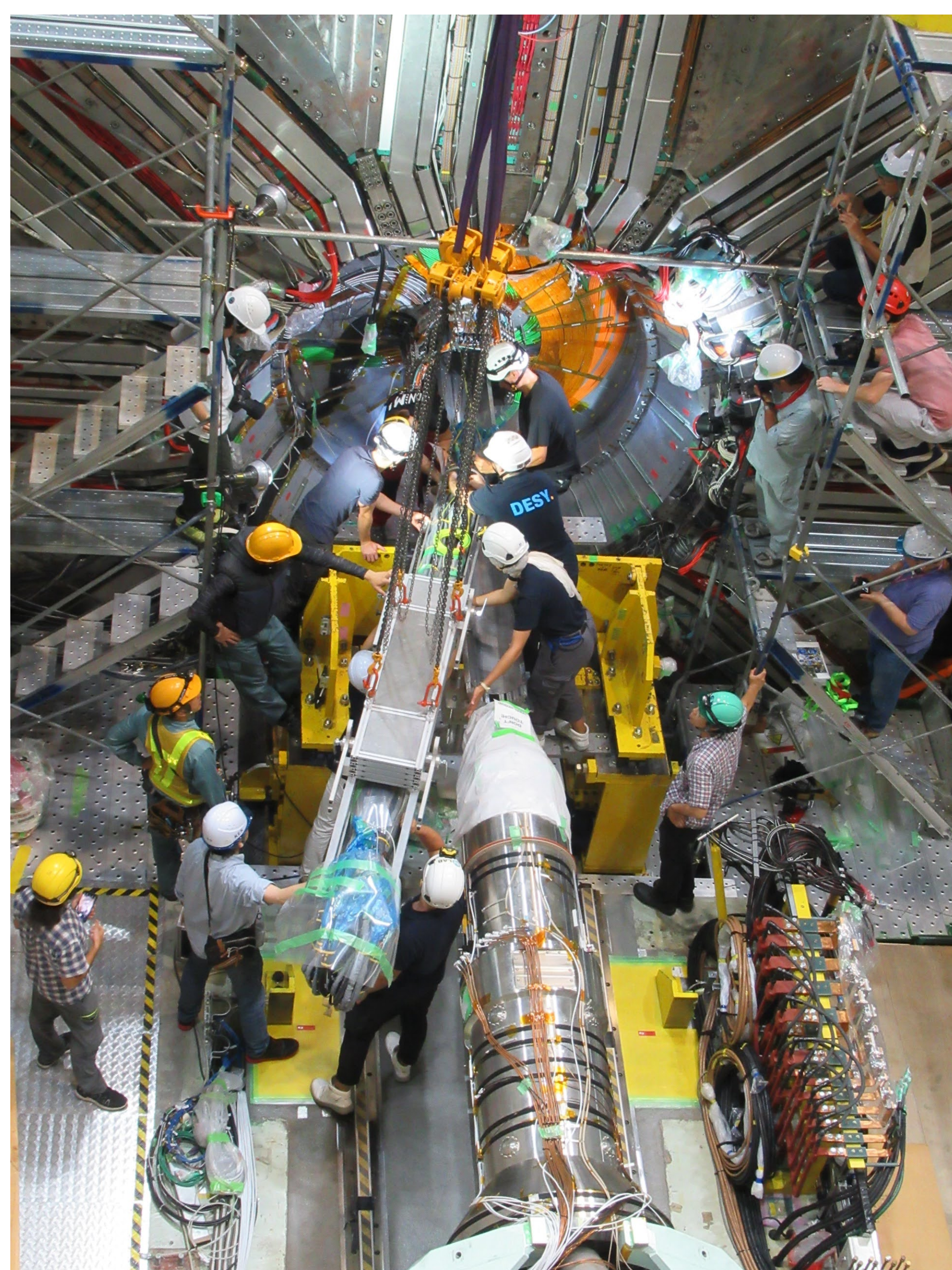
Installation of VXD in Belle 2
