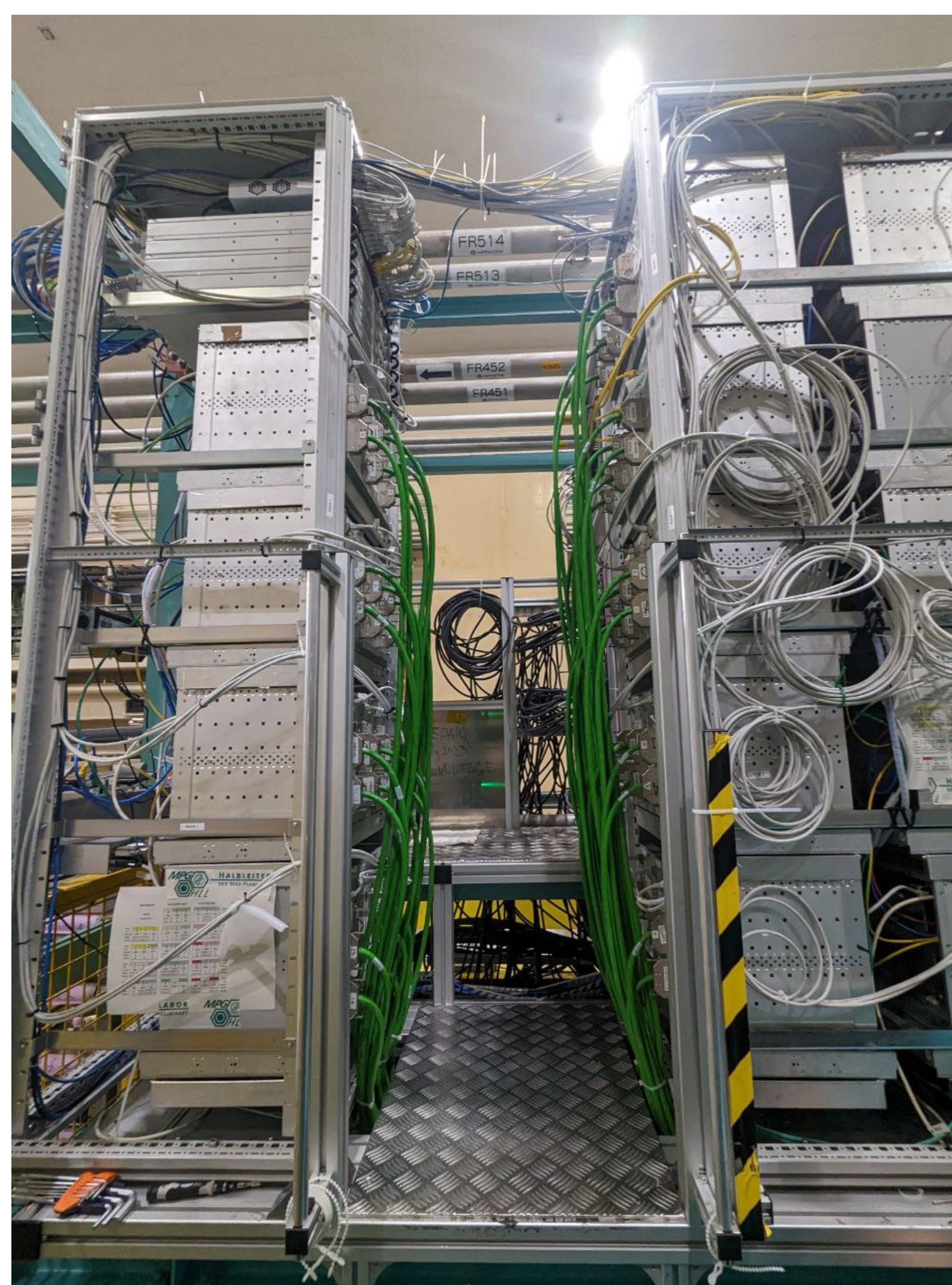
Installation of PXD2 services
