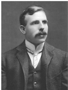
Rutherford
